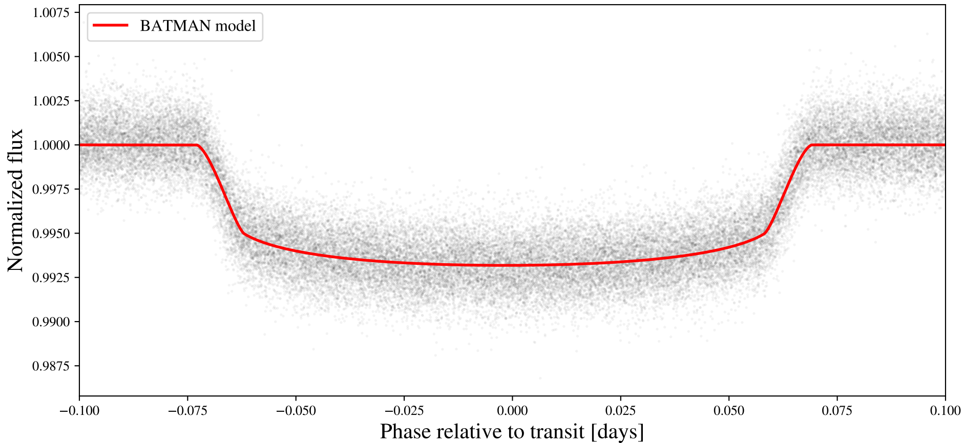
TIC 25155310 — Final MCMC Transit Model
